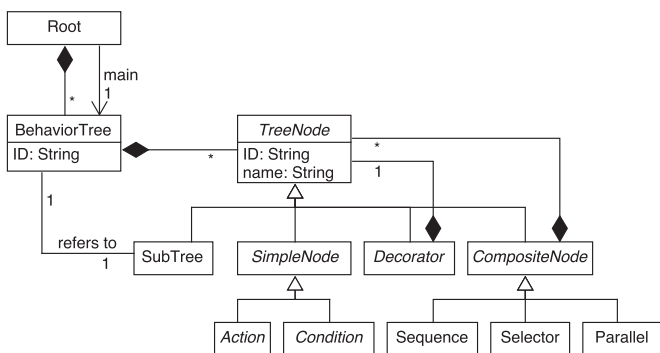
Fig. 6. A meta-model for Behavior-Tree.CPP (reverse-engineered from its XML format)
