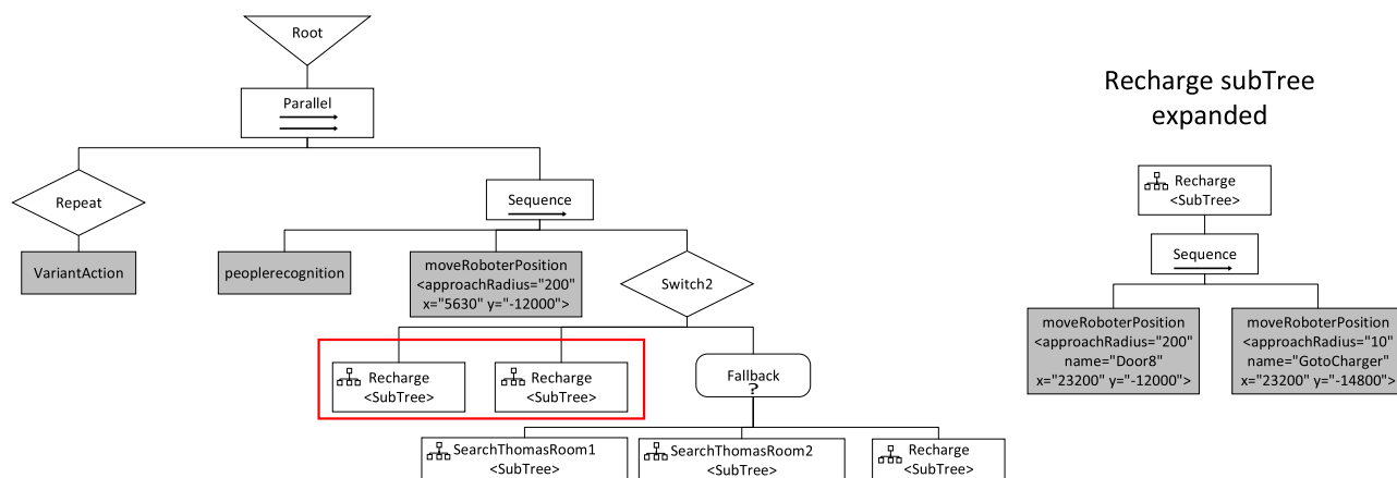
Fig. 10. Behavior tree model of a retirement home robot from project bundles. The red box highlights an example of an intra-model referencing for a sub-tree Recharge (expanded on the right side). A legend is shown in Fig. 2.
