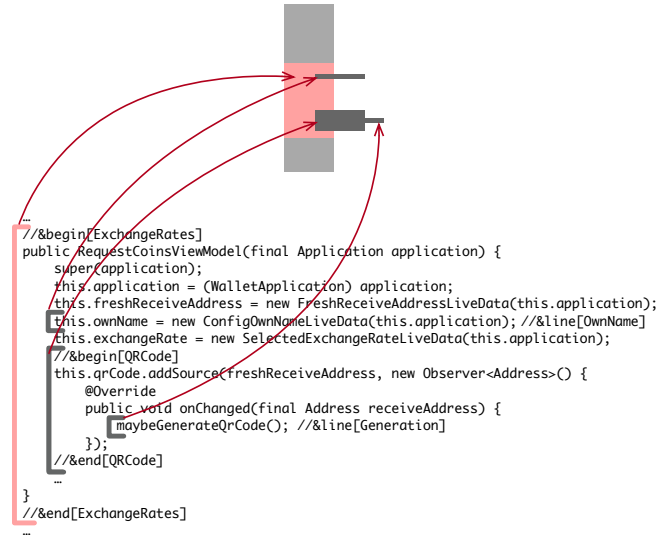
Figure 4: Class glyph
